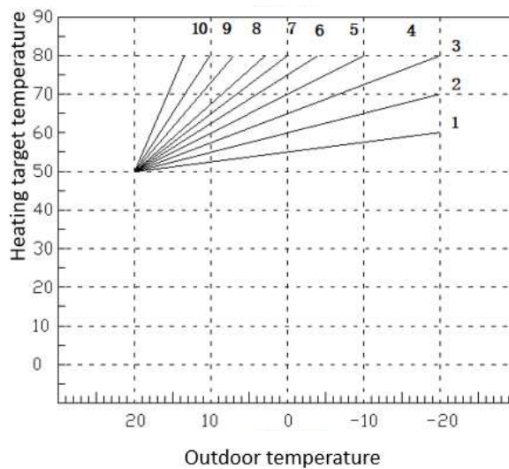
Compensation curve (offset =50)
