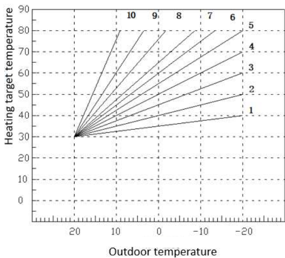
Compensation curve (offset =30)
